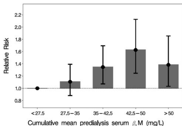
Figure 5. Association of all-cause mortality with cumulative mean predialysis serum \beta_2 M levels. Mean predialysis serum \beta_2 M levels over the follow-up period correlated significantly with mortality ( n = 1813 ; P = 0.001 ) with an apparent plateau phase beyond \beta_2 M levels of 42.5 to 50 mg/L. The statistical analysis was performed using time-dependent Cox regression, adjusted for age, gender, race, diabetes, years on dialysis, serum albumin level, ICED score, residual kidney urea clearance, dialyzer flux, ultrafiltration volume normalized by body weight, and kinetically modeled urea distribution volume, all obtained at baseline, and stratified by clinical center.
