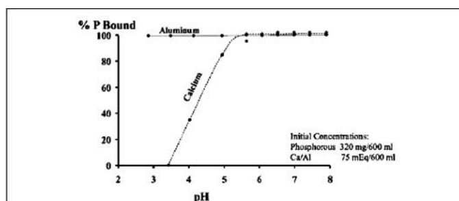
Figure 1. Theoretical analysis of the effect of pH on the binding of phosphorus by dissolved calcium or aluminum at equilibrium. Aluminum bound virtually all the phosphorus regardless of pH, whereas optimal calcium binding required a pH >5 (initial concentrations: phosphorous 320 mg/600 mL; calcium or aluminum 75 mEq/600 mL; adapted from Sheikh et al.). 25
