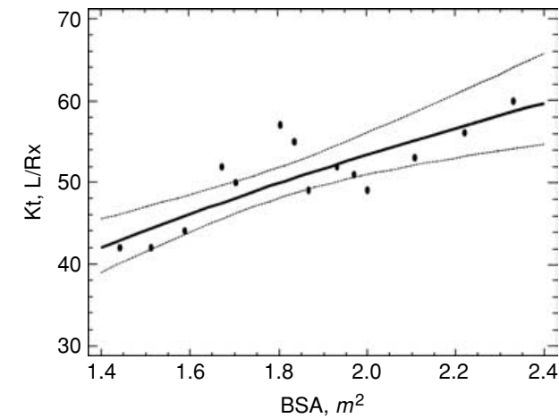
Fig. 6. The best-fit (double reciprocal) to Kt target for each BSA quintile and decile by the mean of BSA for that quintile or decile. The dark solid line is the best-fit relationship. The inner dashed lines indicate the 95% confidence interval for the regression. The standard error of estimates was 3.2 L/treatment, that is, 6.3% of the mean Kt at the mean BSA. See Table 2 for other regression statistics.
