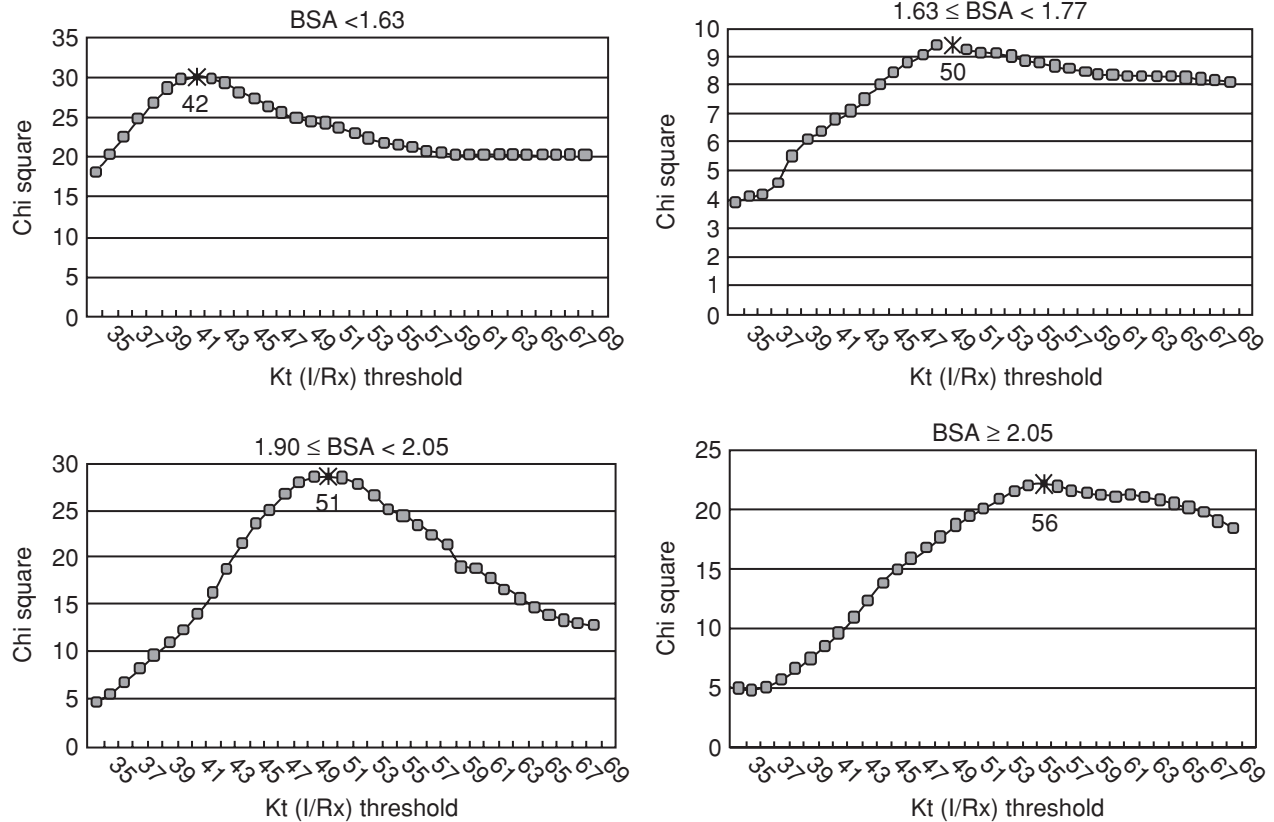
Fig. 3. Death hazard fit curves by Kt target for the 1st, 2nd, 4th, and 5th quintiles of BSA. The best-fit target for the first through fifth quintiles were 42 L/treatment, 50, 55 (curve not shown), 51, and 56, respectively.
