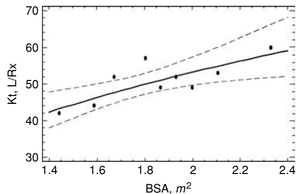
Fig. 5. The best-fit (reciprocal X) to Kt target for each BSA decile by the mean of BSA for that decile. The dark solid line is the best-fit relationship. The dashed lines indicate the 95% confidence interval for the regression. The standard error of estimates was 3.7 L/treatment, that is, 7.3% of the mean Kt at the mean BSA. See Table 2 for other regression statistics.
