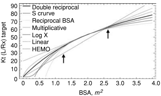
Fig. 7. Comparison of extrapolated curves for the double reciprocal (thick, black curve), S-curve (thick, dark gray curve), reciprocal X (thin, gray curve), multiplicative (thick, light gray curve), and log X (thin, black curve) forms. The linear form for these data is also shown (thin, dash—dot—dash line). A linear, 0-intercept form taken from a regression of the mean BSA and mean Kt for males and females in the standard treatment arm of the HEMO study [30] through the 0,0 origin is provided for comparison (thin, dashed line). The vertical arrows indicate the approximate 98% distribution interval of BSA.
